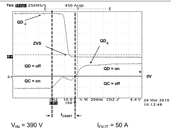
Figure 8-18. Full-Bridge Gate Drives and Switch Nodes (QD g QD d ) ZVS maintained from 50% to 100% output power
