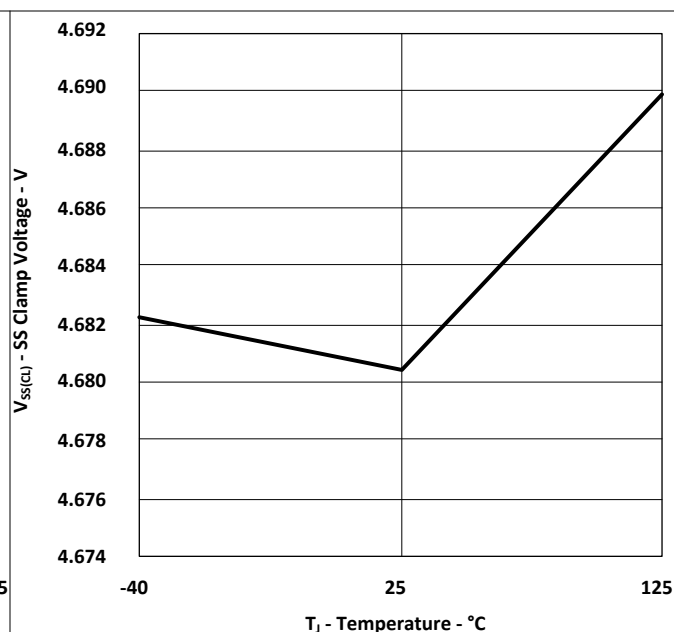
Figure 6-18. SS Clamp Voltage vs Temperature
