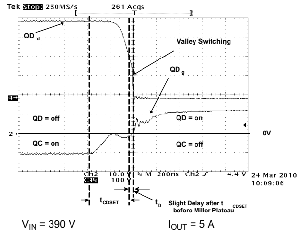
Figure 8-12. Full-Bridge Gate Drives and Primary Switch Nodes (QD g QD d )
