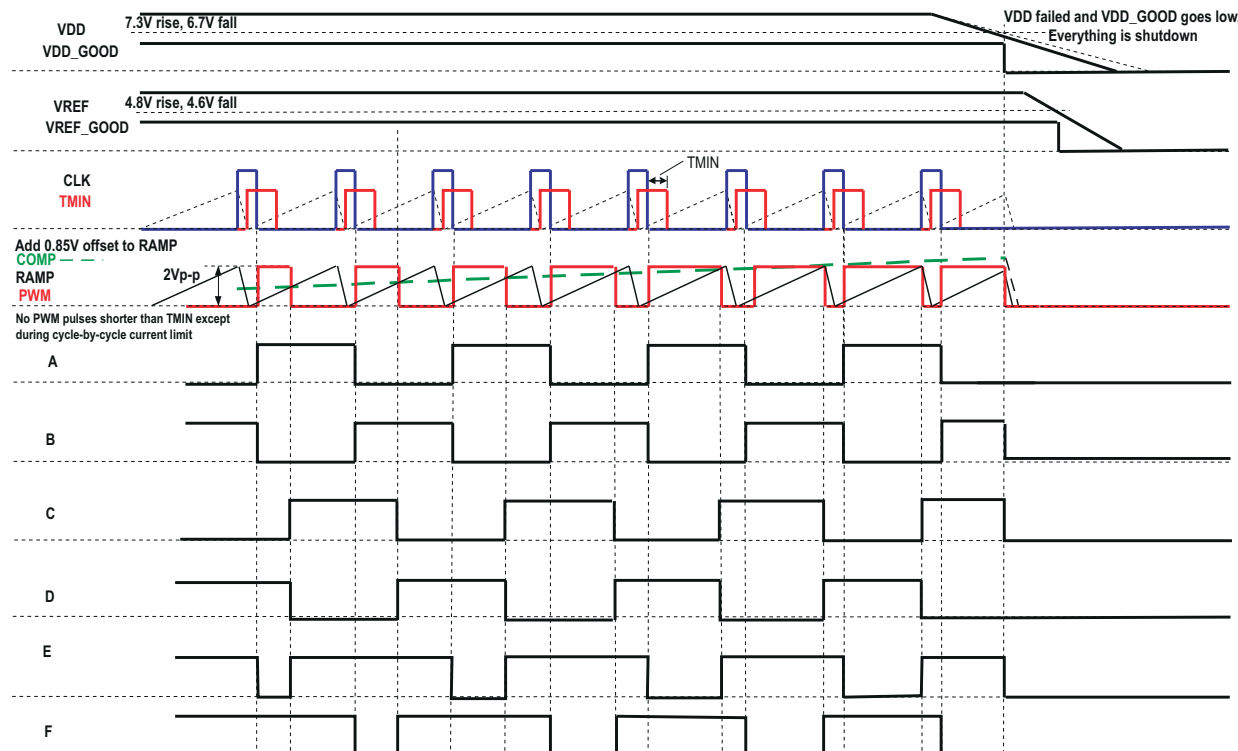
Figure 6-2. UCC28951-Q1 Steady-State and Shutdown Timing Diagram
