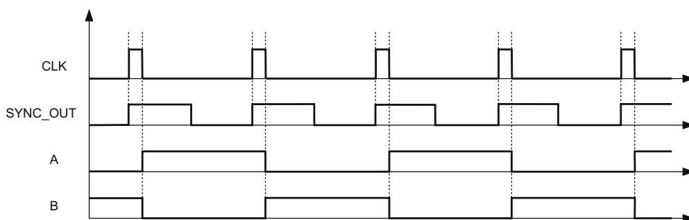
Figure 7-16. SYNC_OUT (leader Mode) Timing Diagram
