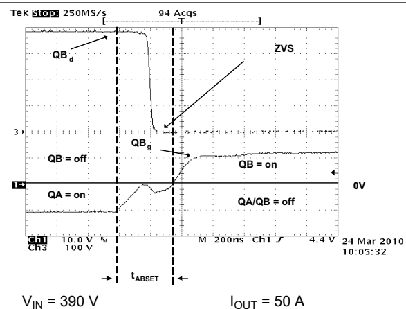
Figure 8-17. Full-Bridge Gate Drives and Switch Nodes (QB g QB d )
