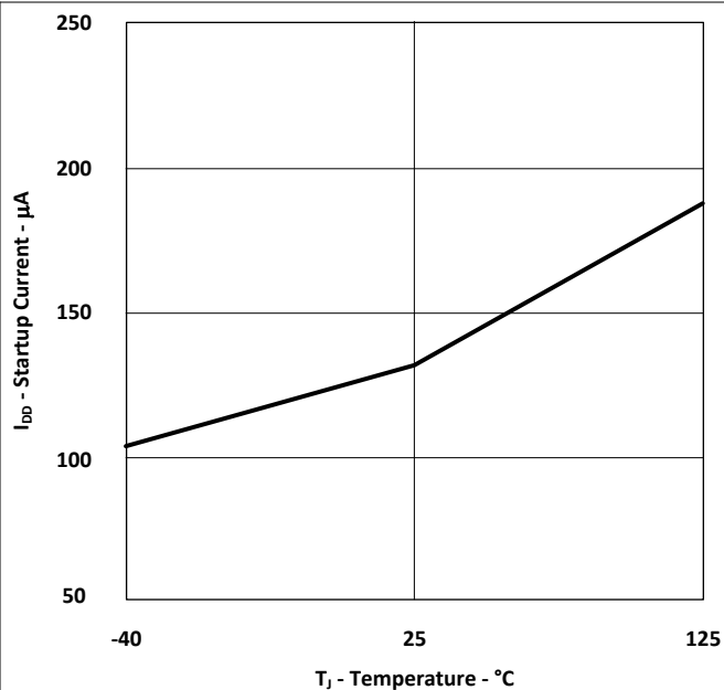
Figure 6-6. Start-Up Current vs Temperature
