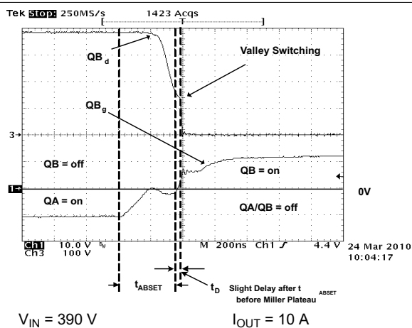
Figure 8-13. Full-Bridge Gate Drives and Switch Nodes (QB g QB d )
