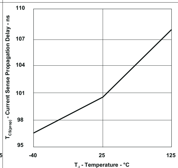
Figure 6-20. Current Sense Propagation Delay vs Temperature
