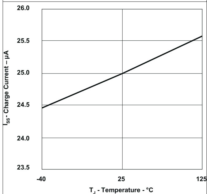
Figure 6-15. I SS Charge Current vs Temperature
