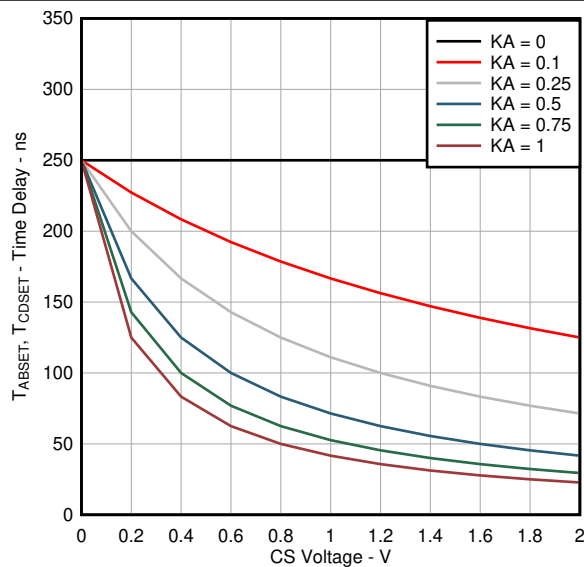
Figure 7-2. Delay Time Set T_{ABSET} and T_{CDSET} (Over CS Voltage Variation and selected K_A for R_{AB} and R_{CD} Equal 13 k \Omega )
