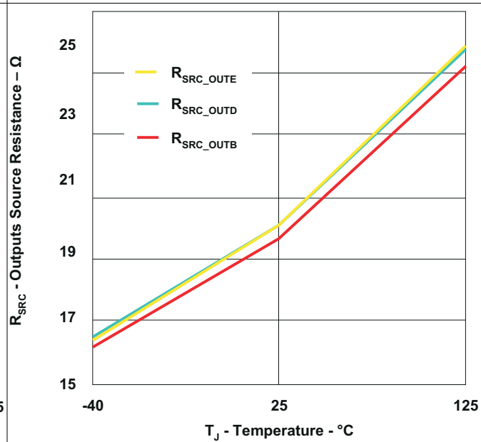
Figure 6-24. Outputs Source Resistance vs Temperature
