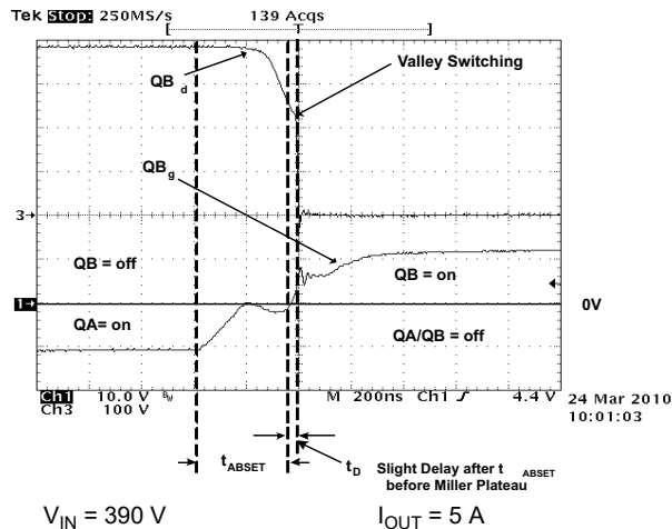
Figure 8-11. Full-Bridge Gate Drives and Primary Switch Nodes (QB d and QD d )
