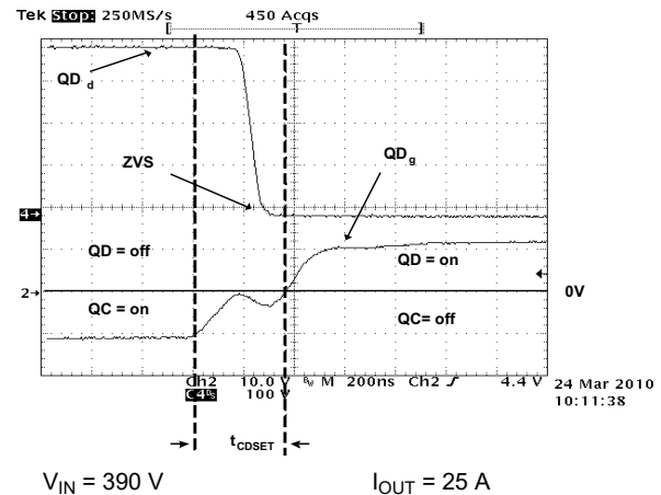
Figure 8-16. Full-Bridge Gate Drives and Switch Nodes (QD g QD d )
