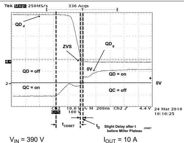
Figure 8-14. Full-Bridge Gate Drives and Switch Nodes (QD g QD d )
