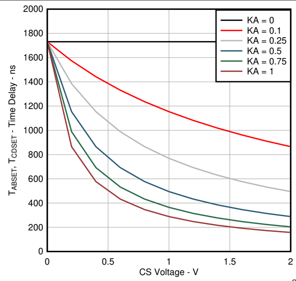
Figure 7-3. Delay Time set T_{ABSET} and T_{CDSET} (Over CS Voltage Variation and Selected K_A for R_{AB} and R_{CD} Equal 90 k \Omega )
