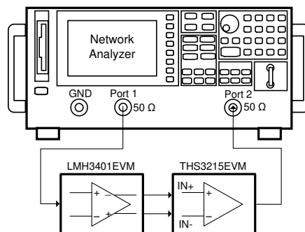
图 7-2. Frequency-Response Measurement: D2S and Full-Path (D2S + OPS) Circuit Configurations
