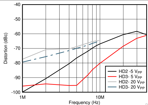
图 9-5. Harmonic Distortion Performance of the 5 V PP and 20 V PP Channels
